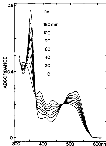
Figure 4. Repetitive spectral scans during the aerobic decomposition of neopentylcobalamin (30 \mu\text{M} ) in 0.10 M phosphate (Na + ) buffer (pH 7.0). The final spectrum was recorded after photolysis of the remaining neopentylcobalamin.
