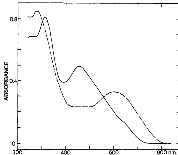
Figure 3. Absorption spectra of benzylcobalamin in acidic (—) and neutral (---) solutions (40 \mu M).
