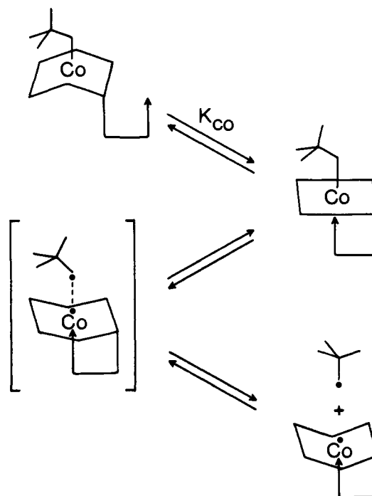
Figure 5. Schematic representation of the corrin conformational changes in the axial base induced homolytic Co-C bond cleavage of neopentylcobalamin.
