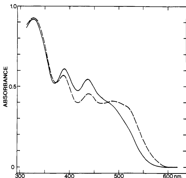
Figure 2. Absorption spectra of neopentylcobalamin in acidic (—) and neutral (---) solutions (60 \mu M).
